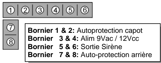
Figure 2: Connexions raccords
